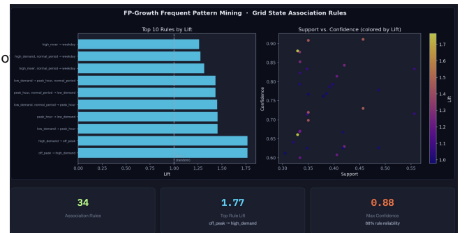
Figure 5: FP-Growth results. Left: top 10 rules by lift; the off_peak \Rightarrow high_demand rule (lift = 1.77) is the strongest. Right: support vs. confidence scatter colored by lift, showing that high-confidence rules cluster at support 0.33–0.45.
